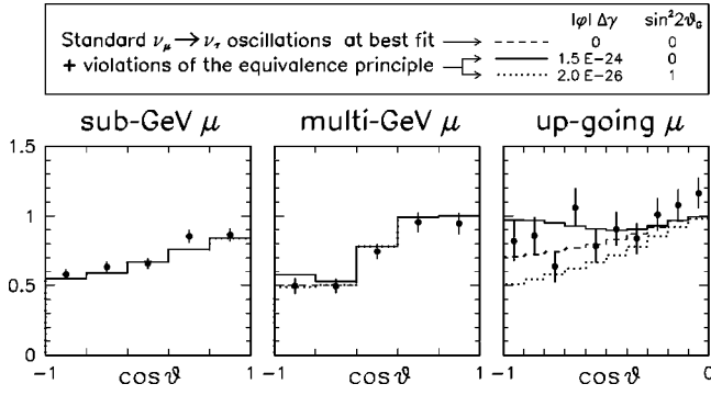
FIG. 5. Effect of subleading oscillations induced by violations of the equivalence principle on the muon distributions in Super-Kamiokande. Standard mass-mixing oscillation parameters are taken at their best fit, and the complex phase e^{i\eta} is taken equal to 1. Dashed line: no VEP. Solid line: VEP with |\phi|\Delta\gamma = 1.5 \times 10^{-24} and \theta_G = 0 . Dotted line: VEP with |\phi|\Delta\gamma = 2 \times 10^{-26} and \theta_G = \pi/4 .
