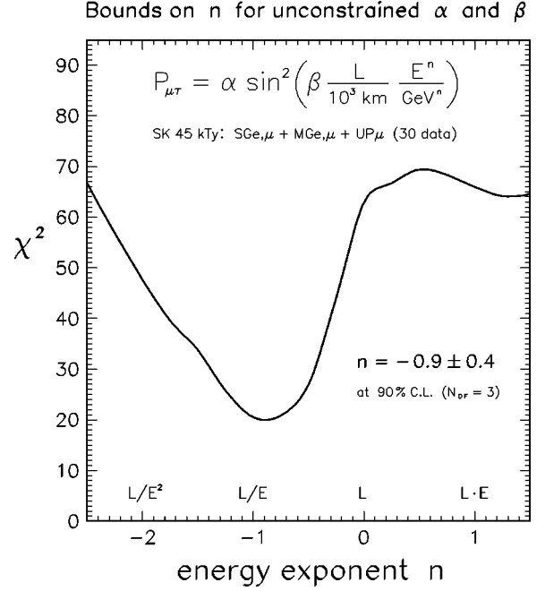
FIG. 3. \chi^2 function from the fit to the SK data, assuming continuous values of the energy exponent n and unconstrained scale factors for the oscillation amplitude \alpha and phase \beta . The standard case ( n = -1 ) is very close to the best fit.
