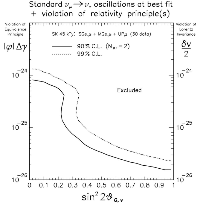
FIG. 6. Bounds on the parameters that characterize violations of special or general relativity principles, assumed to generate subleading \nu_\mu \leftrightarrow \nu_\tau flavor transitions concurrent with standard (leading) neutrino oscillations. Best-fit neutrino mass-mixing values are assumed. See the text for further details.
