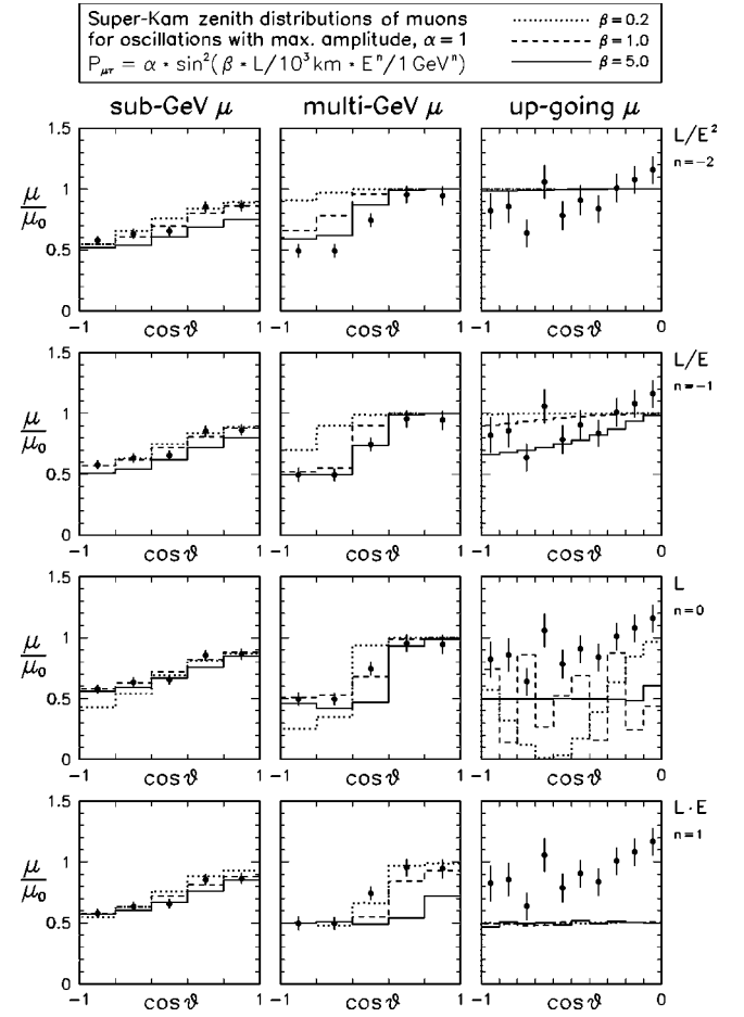
FIG. 1. Expected zenith distributions of SG \mu , MG \mu , and UP \mu events in Super-Kamiokande for maximal mixing ( \alpha=1 ) and for representative values of \beta : dotted line, \beta=0.2 ; dashed line, \beta=1 ; solid line, \beta=5 . In each bin, the muon rates \mu are normalized to the expectations \mu_0 in the absence of oscillations. The 45 kTy SK data (dots with statistical error bars) are superposed to guide the eye. From top to bottom, the energy exponent n takes the values n = -2, -1, 0 , and 1 .
