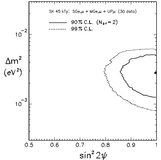
FIG. 4. Updated bounds on the neutrino mass-mixing parameters for standard \nu_\mu \leftrightarrow \nu_\tau oscillations, as derived by our global analysis of all the Super-Kamiokande atmospheric neutrino data.
